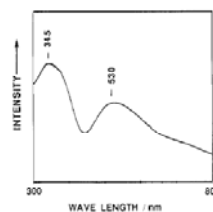
Figure 6. Reflectance spectrum of a solid sample of [\text{Cu}_2(\text{HB}(\text{Ph}(\text{Pr})_2)_3)_2(\text{O}_2) \cdot 3(\text{CH}_2\text{Cl}_2) \cdot 3(\text{C}_2\text{H}_5\text{Cl}_2)] at room temperature.
